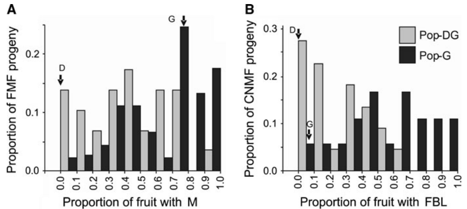
Fig. 2 Phenotypic distribution of a mealiness in two peach cultivars ( D ‘Dr. Davis’; G ‘George Bell’) and in FMF progeny only and b flesh bleeding in the same two cultivars and in CNMF seedlings only. M mealiness; FBL flesh bleeding; FMF freestone melting flesh; CNMF clingstone non-melting flesh
