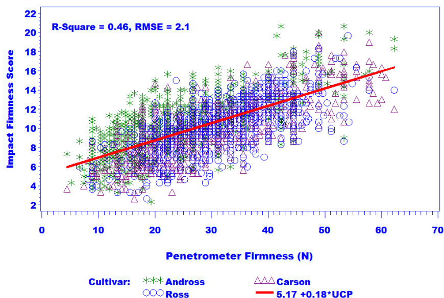
Figure 1. Relationship between impact and penetrometer (UCP) firmness measurements for three clingstone peach cultivars.
